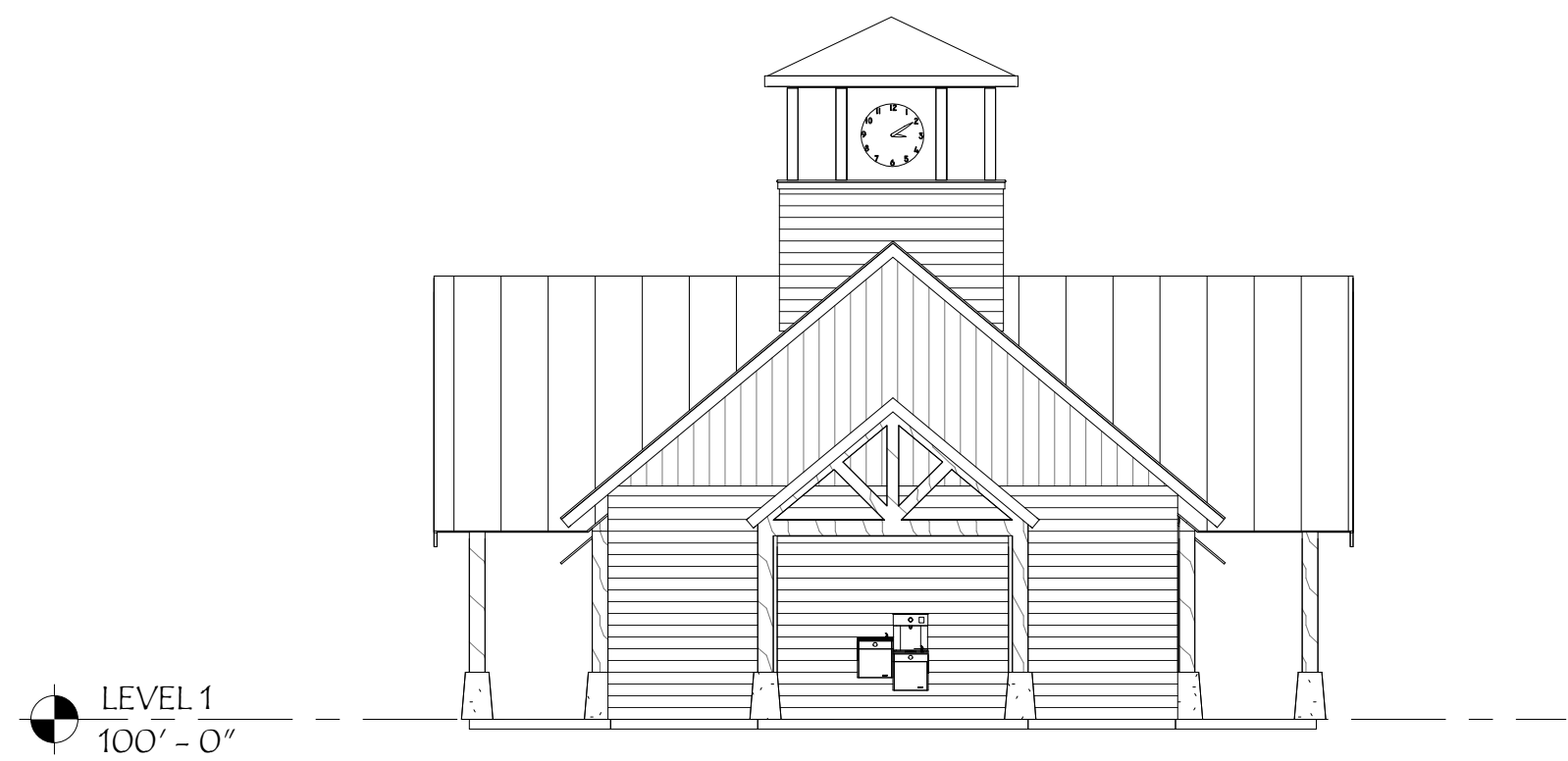
3 LEFT SIDE ELEVATION A1.01 1/8" = 1'-0"
