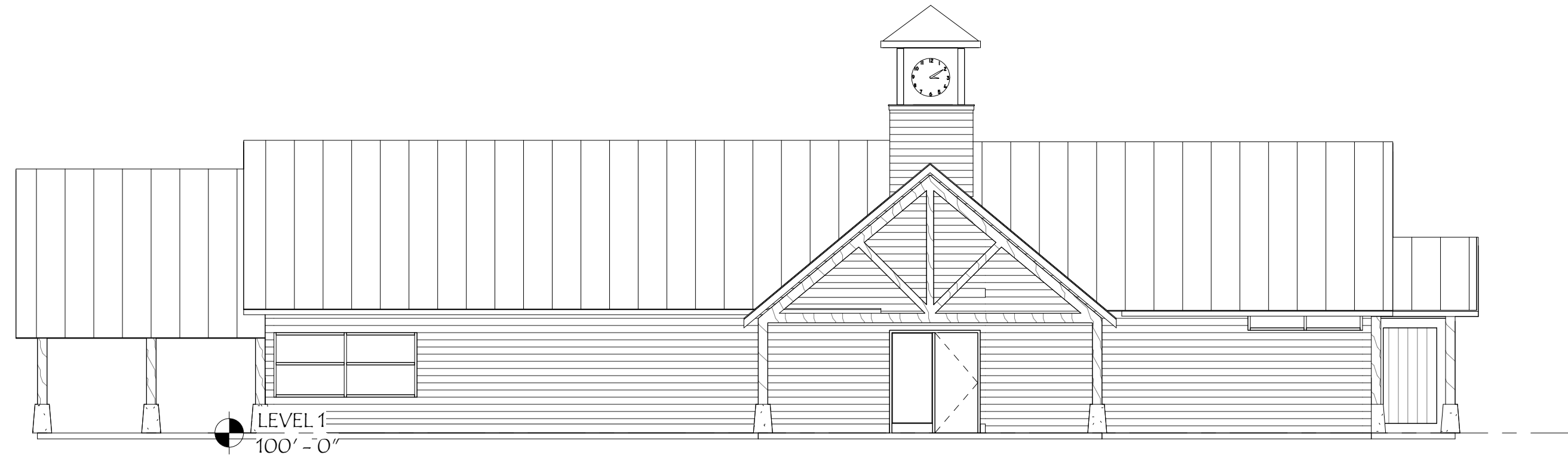
4 REAR ELEVATION A1.01 1/8" = 1'-0"
