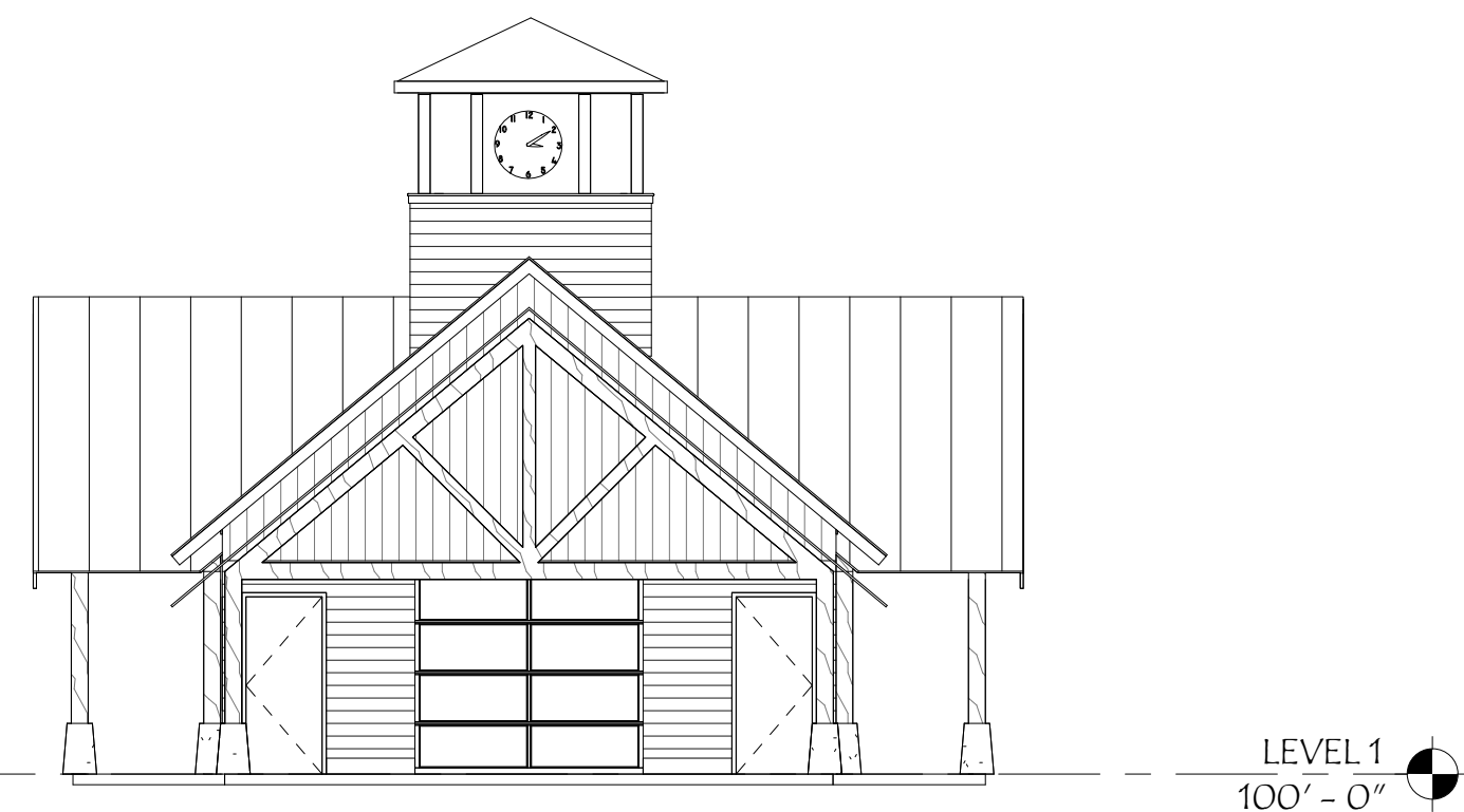
2 RIGHT SIDE ELEVATION A1.01 1/8" = 1'-0"
