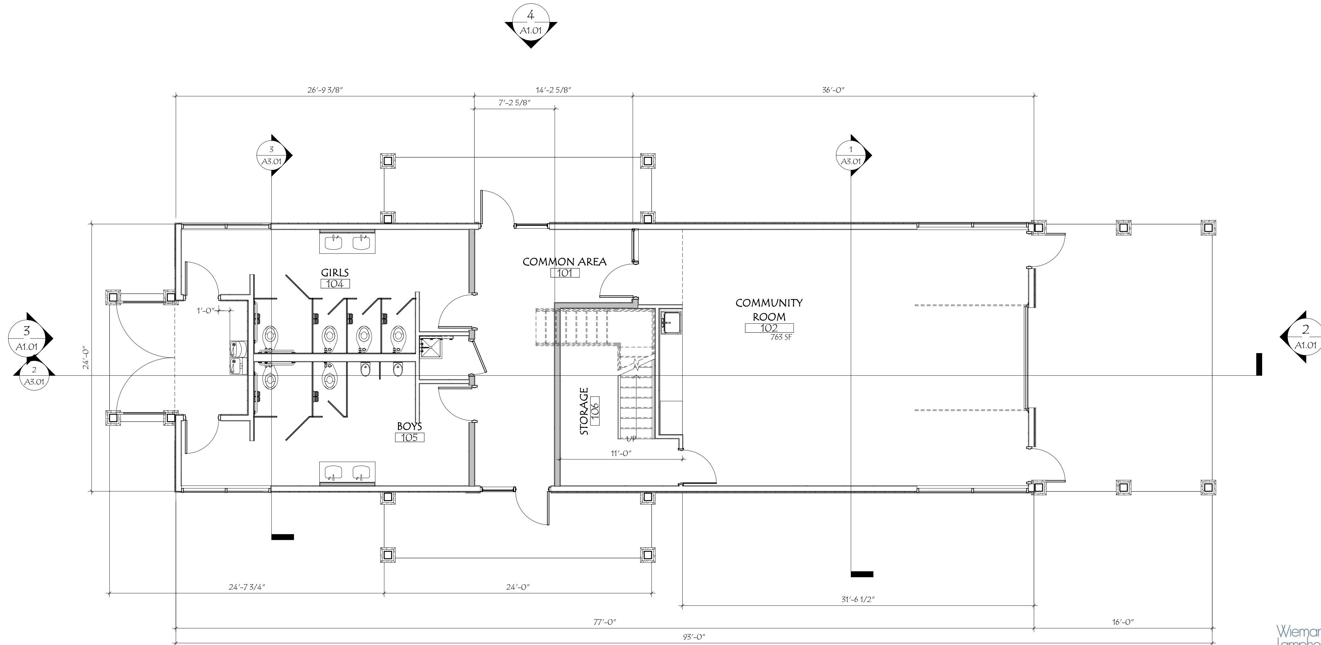
1 FLOOR PLAN A1.01 3/16" = 1'-0"
